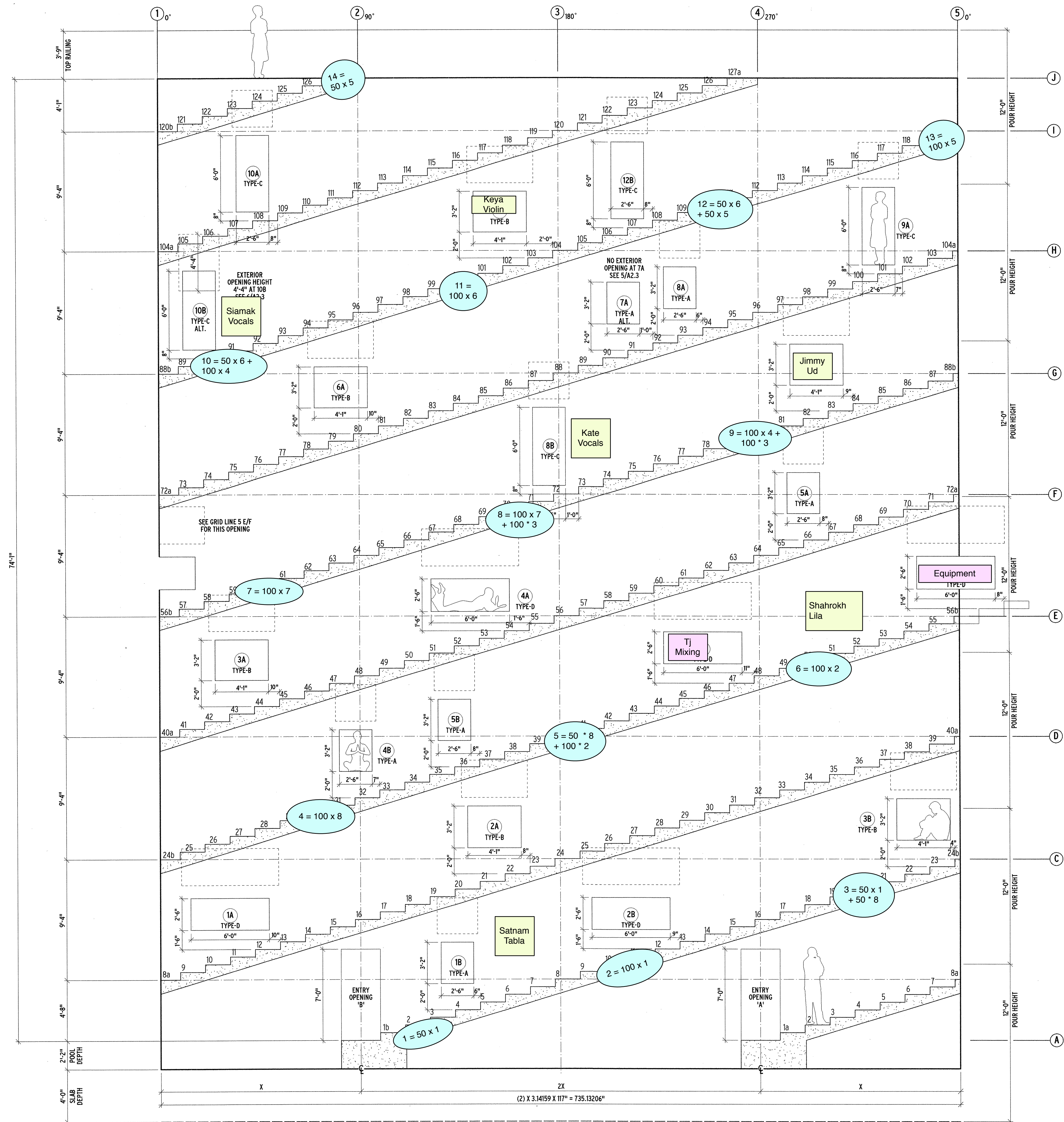
1 UNROLLED ELEVATION (INTERIOR) 1/4" = 1'-0"
